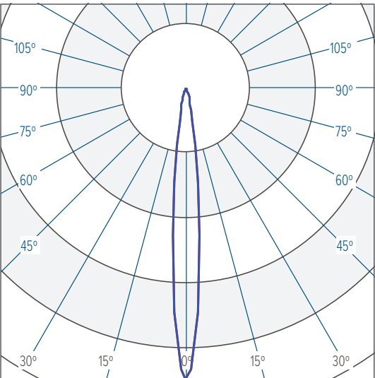
3000K High Output CBCP 83773 @ 5419 lumens
