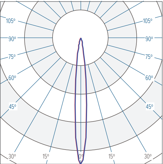
4000K Standard Output CBCP 61598 @ 4127 lumens
