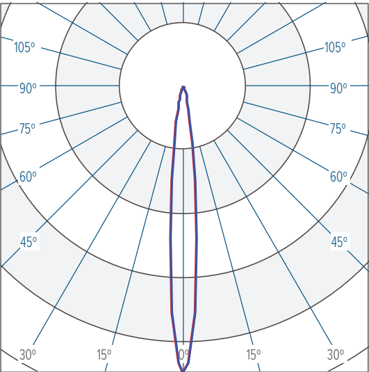
3000K Standard Output CBCP 61598 @ 4127 lumens
