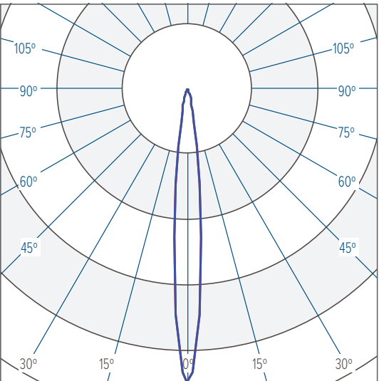
4000K High Output CBCP 83773 @ 5419 lumens
