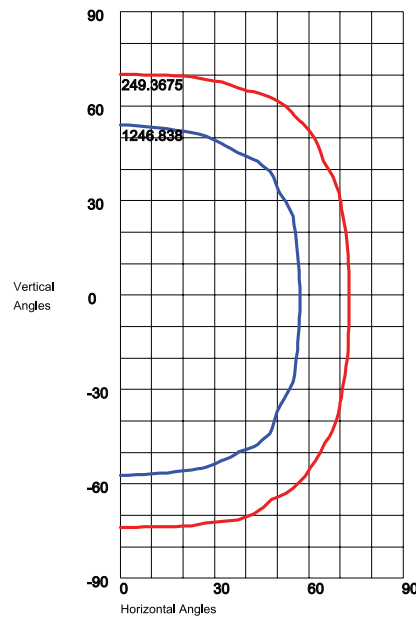
Maximum Candela = 2493.675 Located at Horizontal Angle = 1, Vertical Angle = 3 50% Maximum Candela = 1246.8375 10% Maximum Candela = 249.3675
